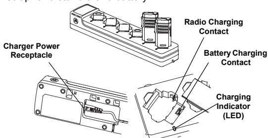
Figure 1: Multi Unit Charger
